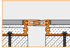
4.24 Schluter®-DILEX-STF
