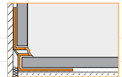
4.13 Schluter®-DILEX-EKE
